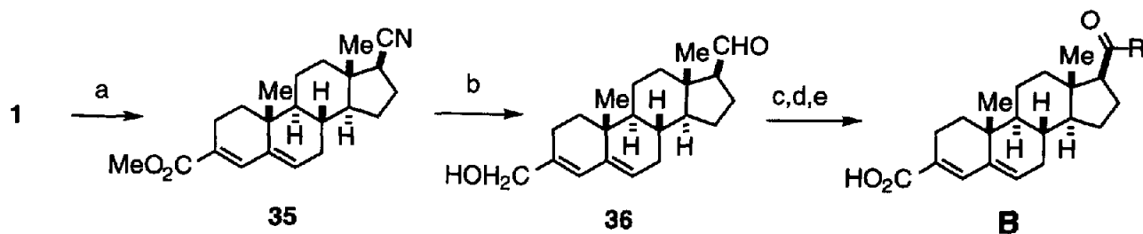
Scheme 2. Synthesis of 20-keto-androsta-3,5-dienes. (a) \text{POCl}_3 , PhMe; MeOH; (b) DIBAL, PhMe; (c) \text{RMgX} , THF; (d) cat. TPAP, NMO, 4 Å sieves, \text{CH}_2\text{Cl}_2 ; (e) \text{NaClO}_2 , THF, \text{H}_2\text{O} , 2-methyl-2-butene.
