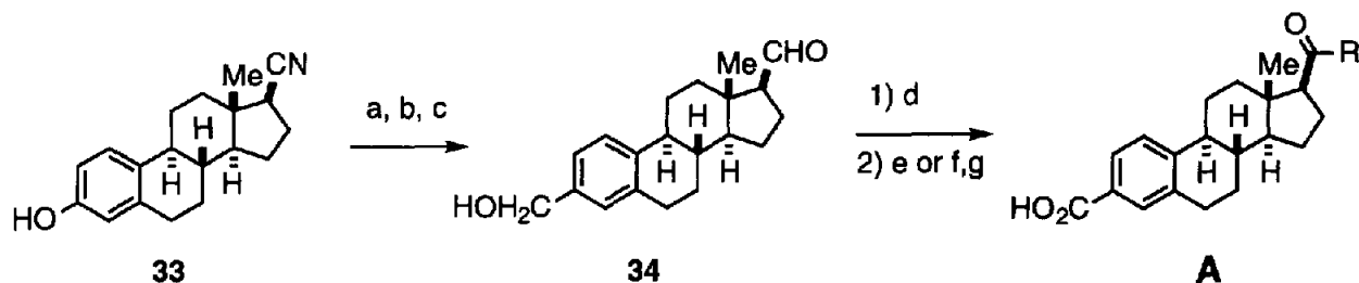
Scheme 1. Synthesis of 20-keto-estra-1,3,5-trienes. (a) \text{PhNTf}_2 , NaH, THF; (b) cat. \text{Pd}(\text{OAc})_2 , CO, dppf, DMF, \text{Et}_3\text{N} , MeOH; (c) DIBAL, PhMe; (d) \text{RMgX} , THF; (e) Jones reagent, acetone; (f) cat. TPAP, NMO, 4 Å sieves, \text{CH}_2\text{Cl}_2 ; (g) \text{NaClO}_2 , THF, \text{H}_2\text{O} , 2-methyl-2-butene.
