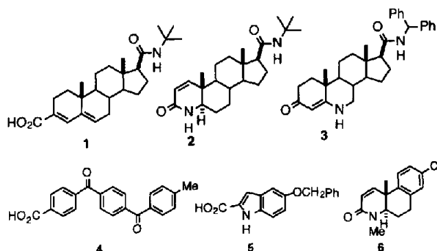
Figure 1. Structural motifs for known steroid 5\alpha -reductase inhibitors.
